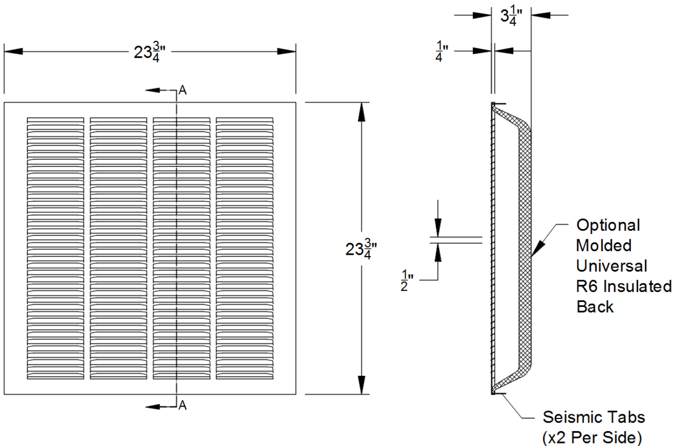
Section AA
