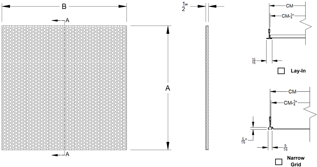
Section AA
